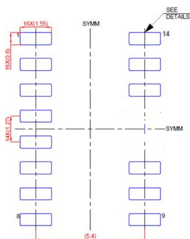
Figure 10.8 SOP14 Package Board Layout Example(mm)
