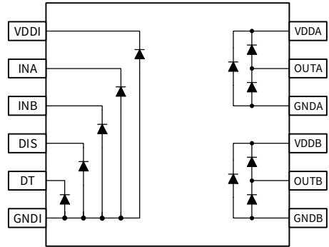
Figure 8.3 ESD Structure
