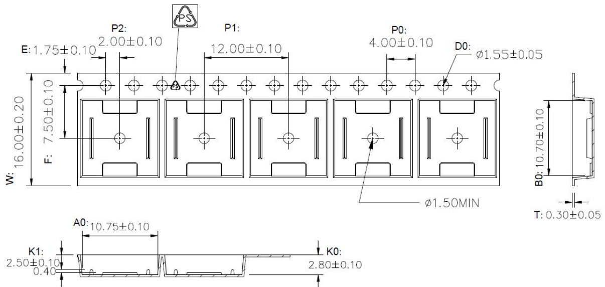
Figure 12.1 Tape Information
