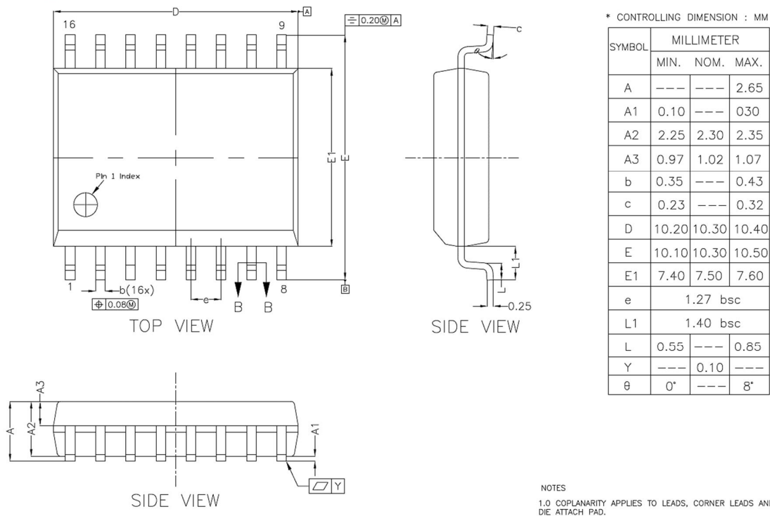
Figure 10.1 SOW16 Package Shape and Dimension
