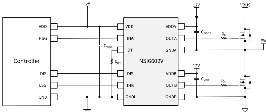
Figure 9.1 Typical Half-Bridge Application Schematic
