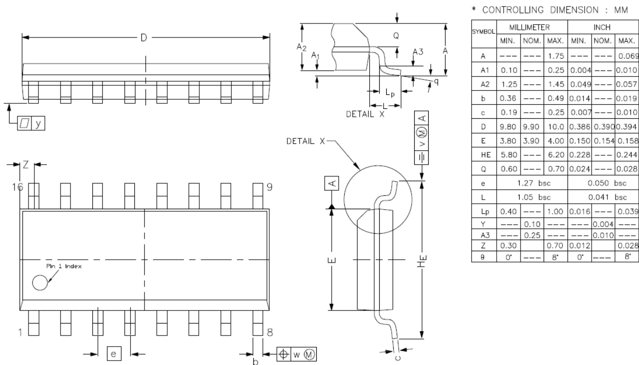
Figure 10.5 SOP16 Package Shape and Dimension
